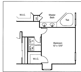
Newbury Optional 5th Bedroom Plan
