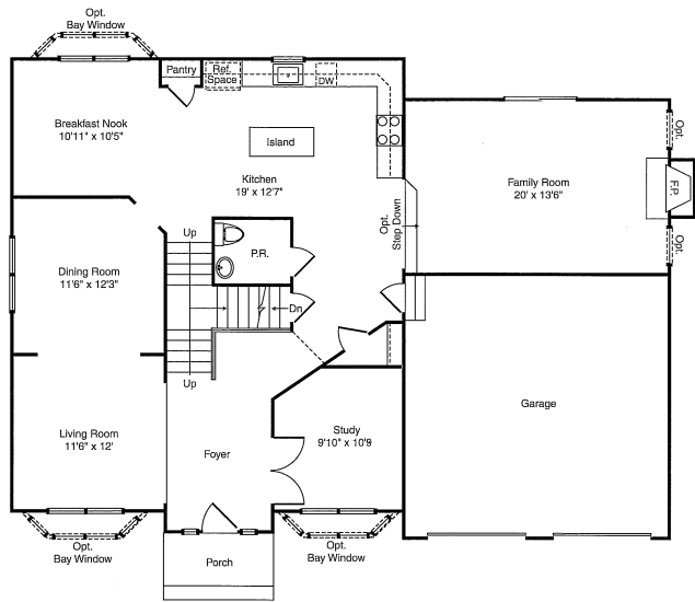
Elevation A First Floor Plan
